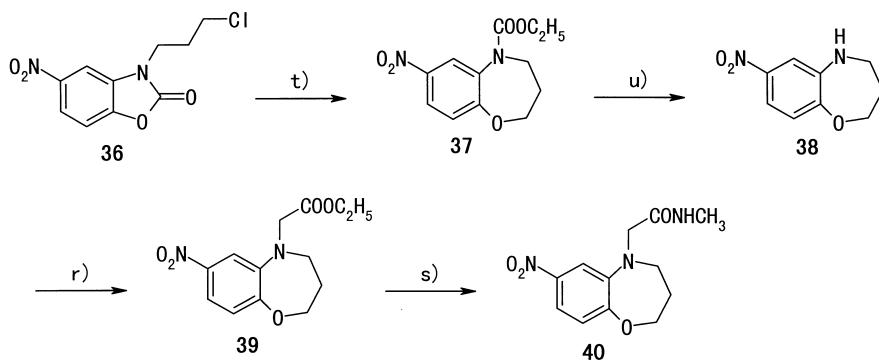
Scheme 6. (t) (i) KOH, EtOH, (ii) DMF, 80 °C; (u) KOH aq ., EtOH, reflux.
