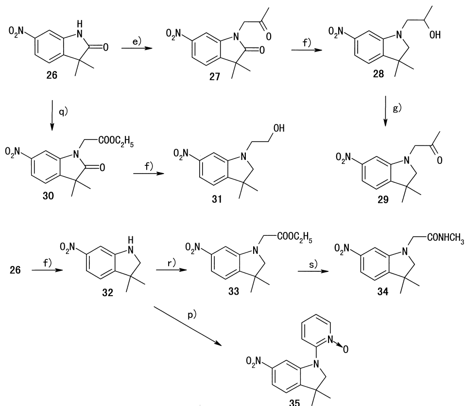
Scheme 5. (q) BrCH 2 COOC 2 H 5 , NaH, DMF; (r) BrCH 2 COOC 2 H 5 , K 2 CO 3 , 100 °C; (s) CH 3 NH 2 , MeOH.
