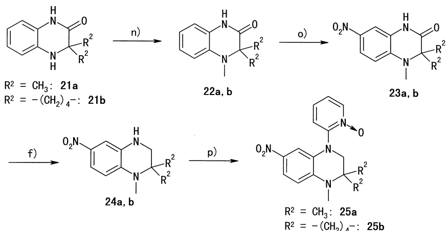
Scheme 4. (n) HCHO, NaBH 3 CN, CH 3 COOH; (o) f. HNO 3 , Ac 2 O; (p) NaH, DMF, 2-bromopyridine 1-oxide hydrochloride.
