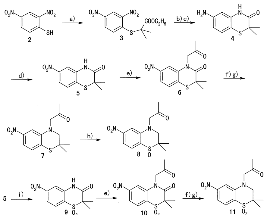
Scheme 2. (a) \text{BrC}(\text{CH}_3)_2\text{COOC}_2\text{H}_5 , \text{K}_2\text{CO}_3 , DMF; (b) Fe, HCl, EtOH; (c) NaOHaq, reflux; (d) (i) \text{NaNO}_2 , \text{H}_2\text{SO}_4 , (ii) \text{NaHCO}_3 , \text{NaNO}_2 , \text{CuSO}_4 , \text{Cu}_2\text{O} ; (e) \text{ClCH}_2\text{COCH}_3 , \text{K}_2\text{CO}_3 , DMF; (f) \text{BH}_3\text{-THF} ; (g) Swern oxidation; (h) m -CPBA; (i) m -CPBA excess.
