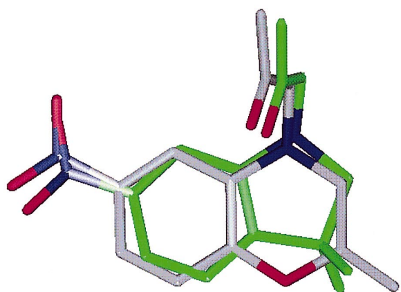
Figure 2. Molecular overlap of compound 1 and 29.
