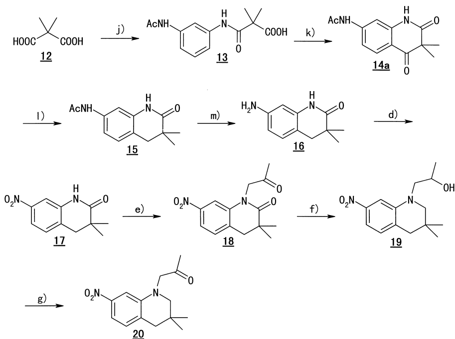
Scheme 3. (j) (i) \text{SOCl}_2 , THF; (ii) 3-aminoacetanilide, \text{Et}_3\text{N} ; (k) polyphosphoric acid; (l) \text{H}_2 , Pd/C, \text{Ac}_2\text{O} , \text{H}_2\text{SO}_4 , AcOH; (m) \text{HClaq.} , EtOH.
